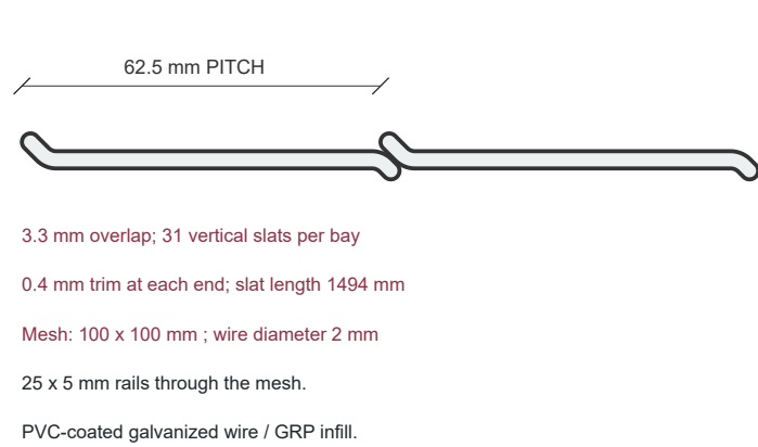
E PANEL ASSEMBLY DETAILS
