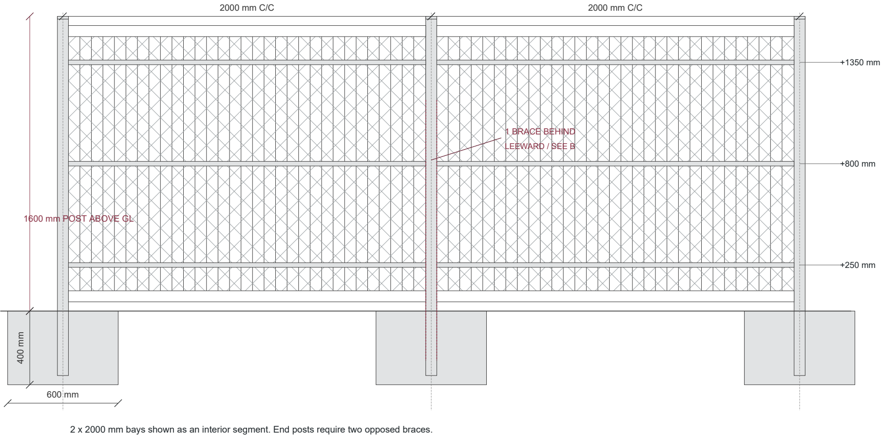
A ELEVATION / BRACE BEHIND 1:20
