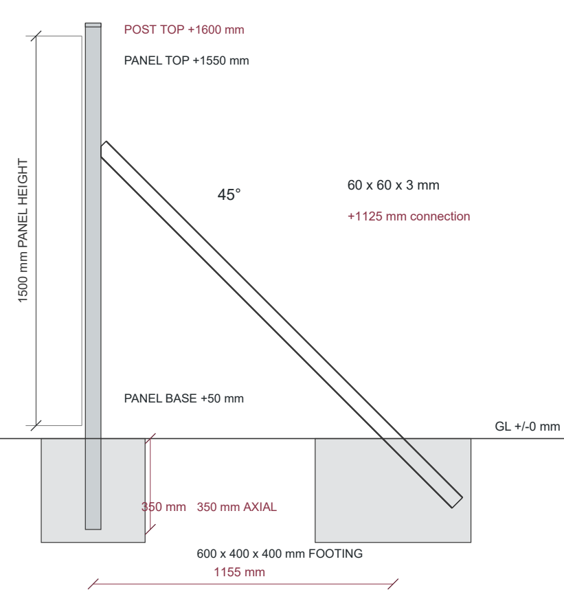
B POST / BRACE SECTION 1:20
